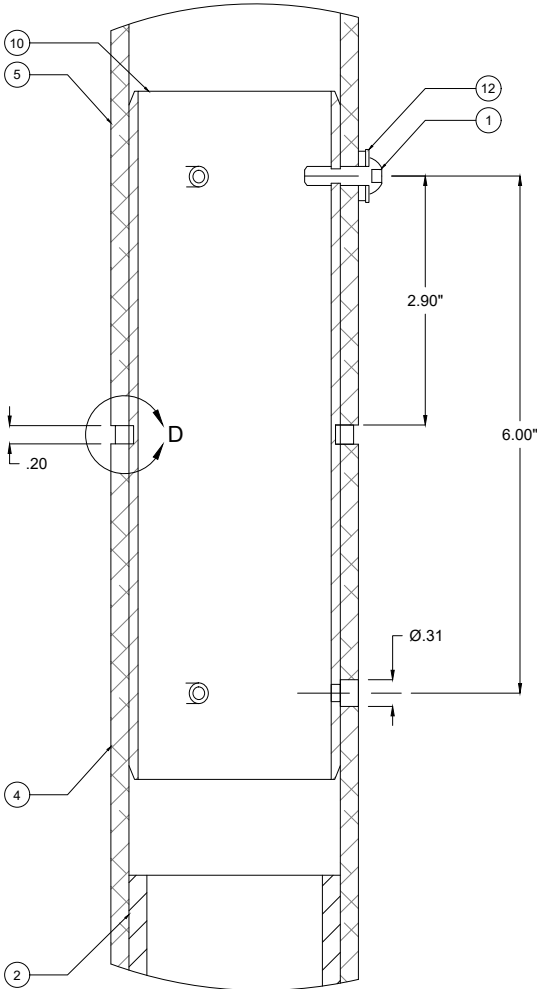
DETAIL B
