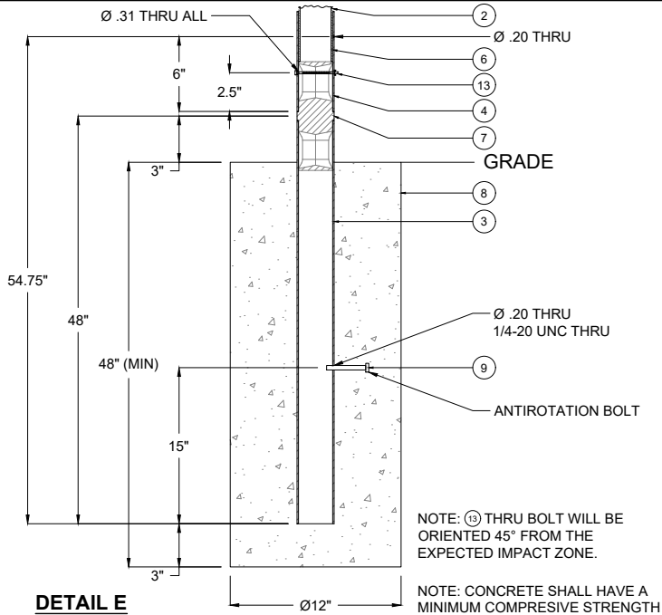
DETAIL E
