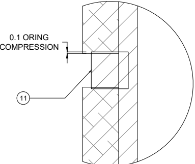
DETAIL D
