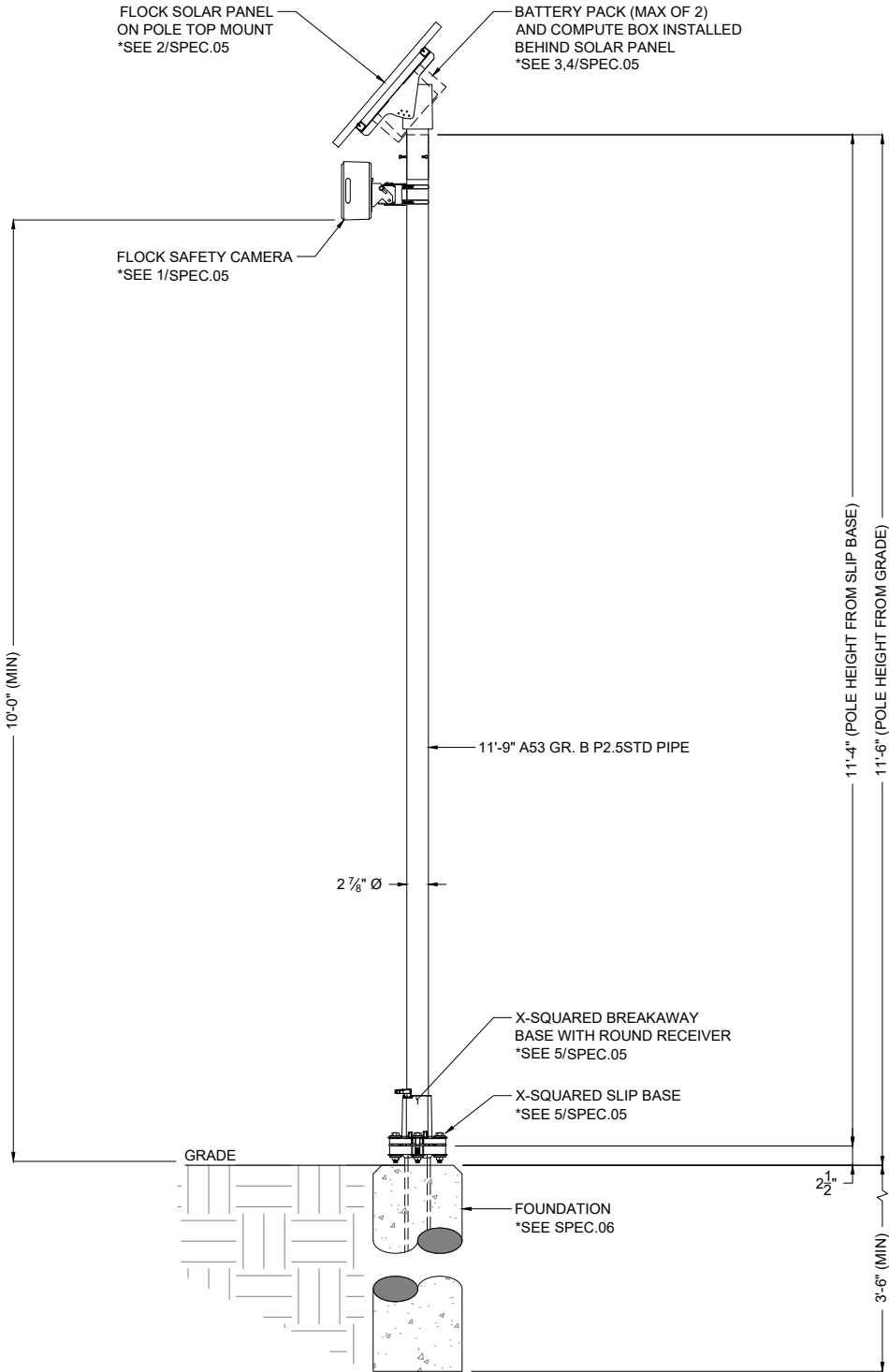
1 POLE ELEVATION DETAIL SCALE: 1:20
