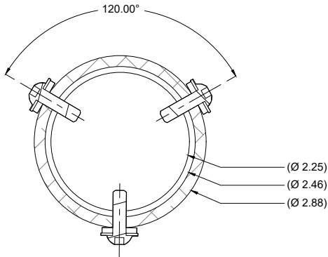
SECTION C-C
